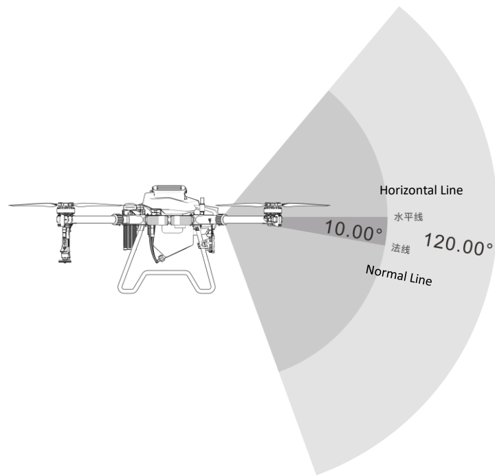
Figure 2-9 Vertical View
