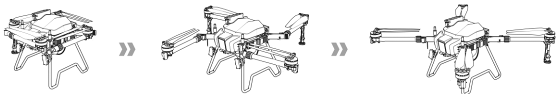
Figure 1-32 Arm Unfolding
